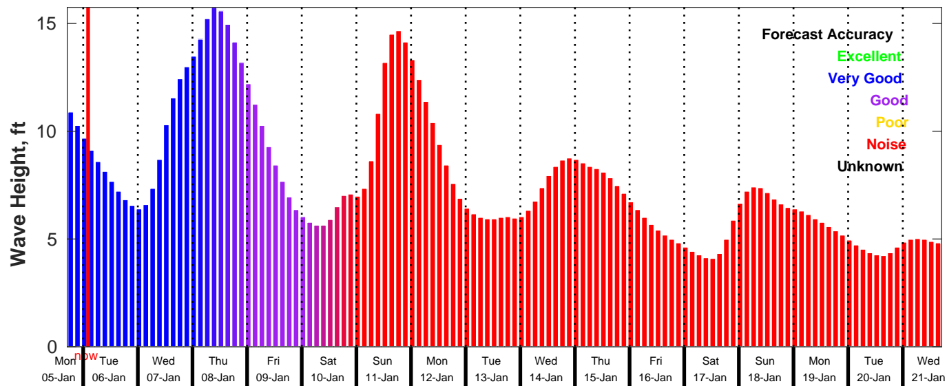
GFS Wave Forecast for NDBC 46059 from 05-Jan-2026 17:00:00 to 21-Jan-2026 17:00:00
