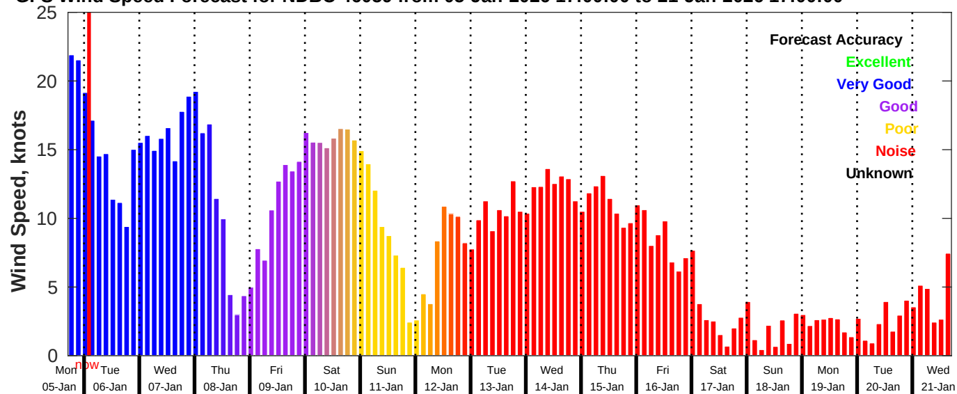
GFS Wind Speed Forecast for NDBC 46059 from 05-Jan-2026 17:00:00 to 21-Jan-2026 17:00:00
