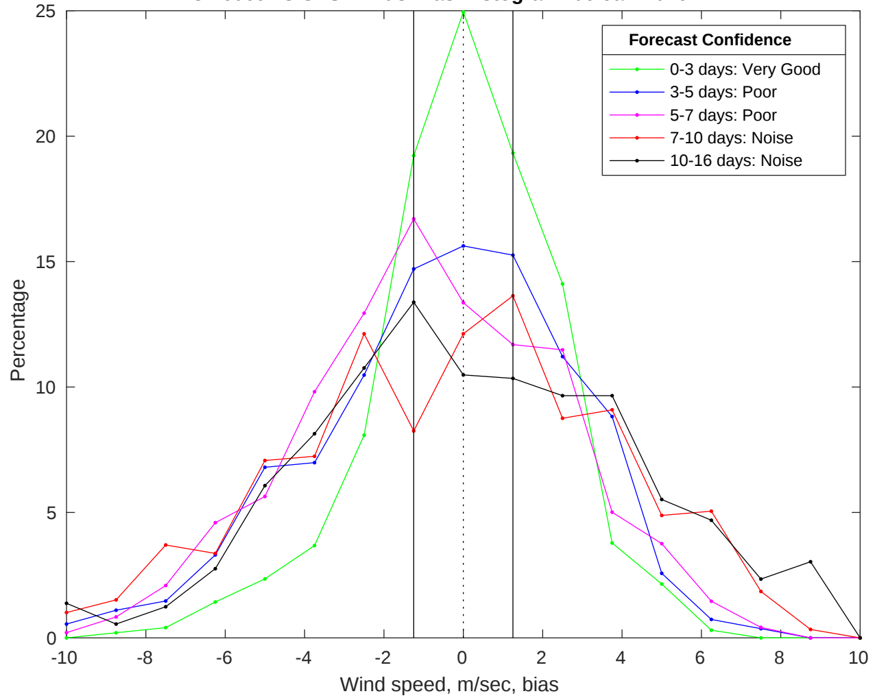
NDBC 46069 vs GFS Winds Bias Histogram: 06-Jan-2026
