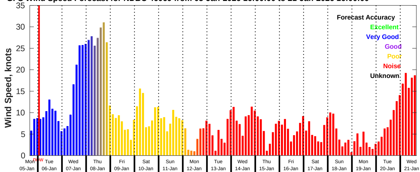
GFS Wind Speed Forecast for NDBC 46069 from 05-Jan-2026 16:00:00 to 21-Jan-2026 16:00:00
