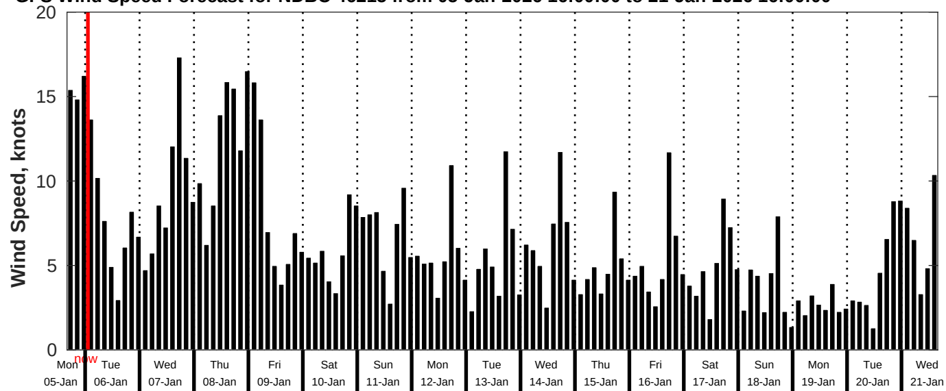
GFS Wind Speed Forecast for NDBC 46215 from 05-Jan-2026 16:00:00 to 21-Jan-2026 16:00:00
