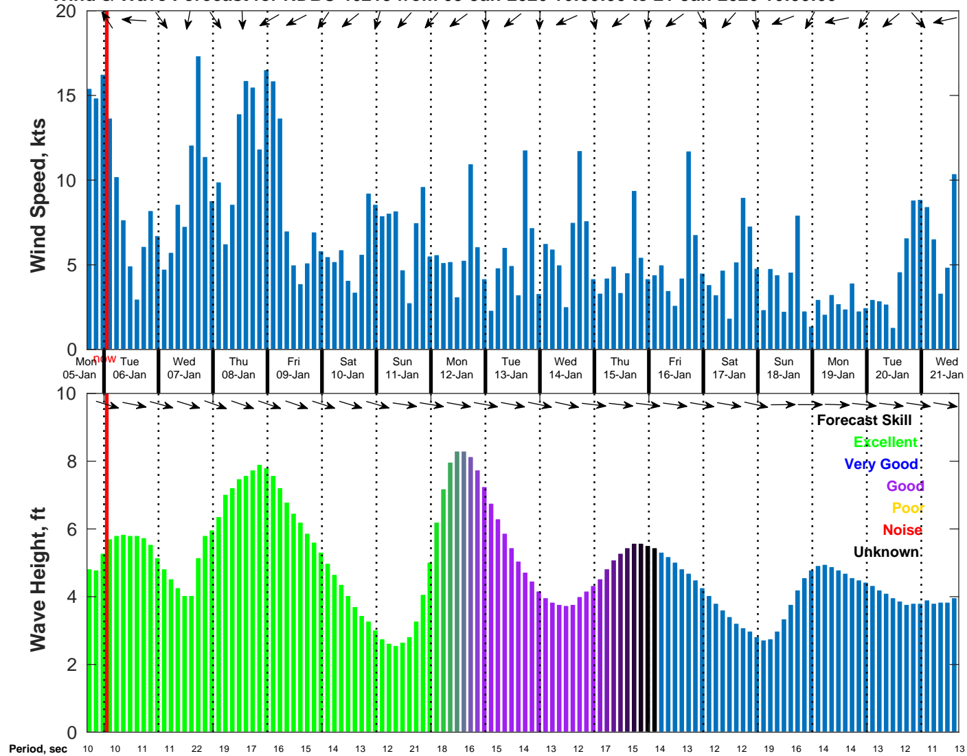
Wind & Wave Forecast for NDBC 46215 from 05-Jan-2026 16:00:00 to 21-Jan-2026 16:00:00
