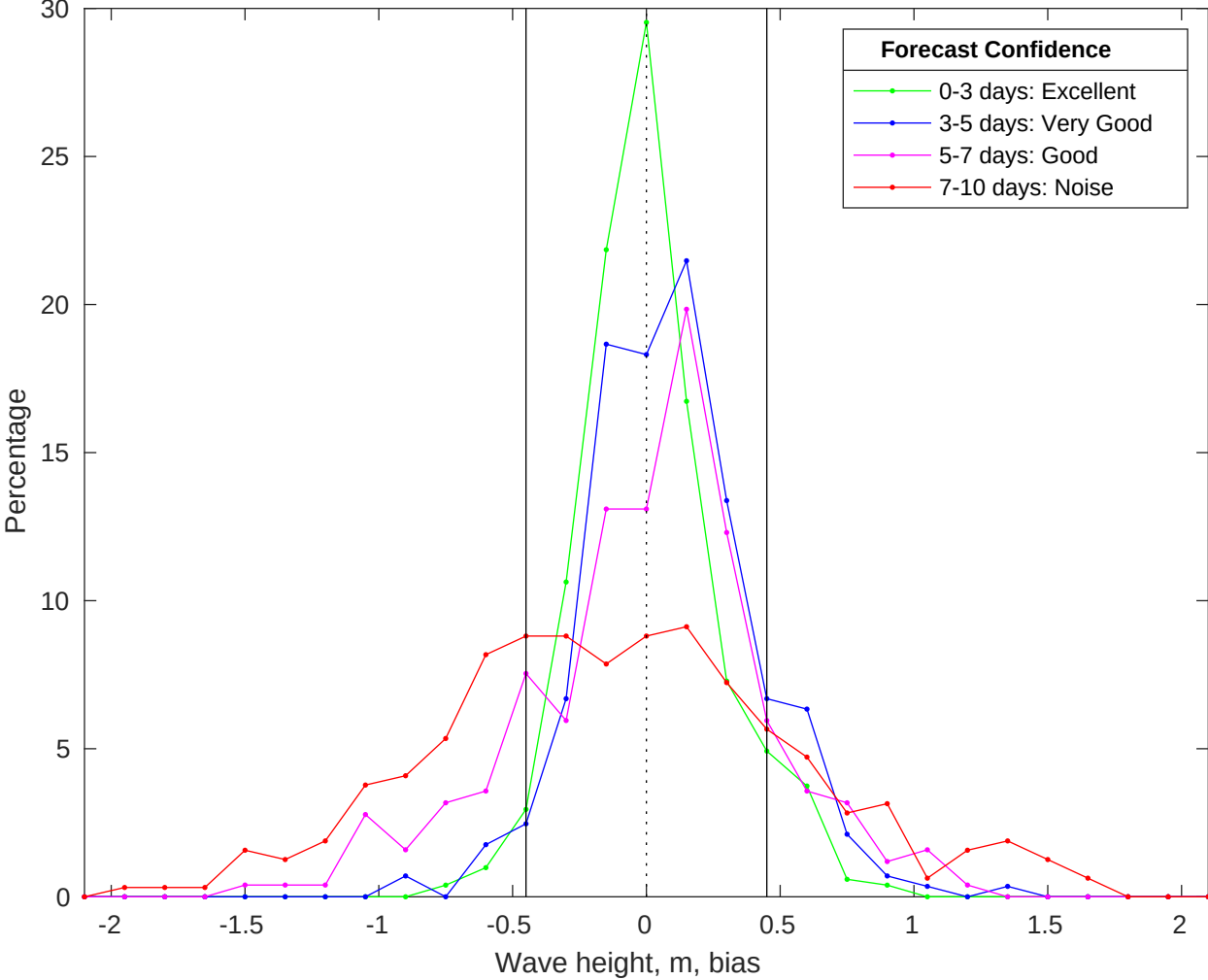
NDBC 46259 vs CMEMS Waves Bias Histogram: 06-Jan-2026
