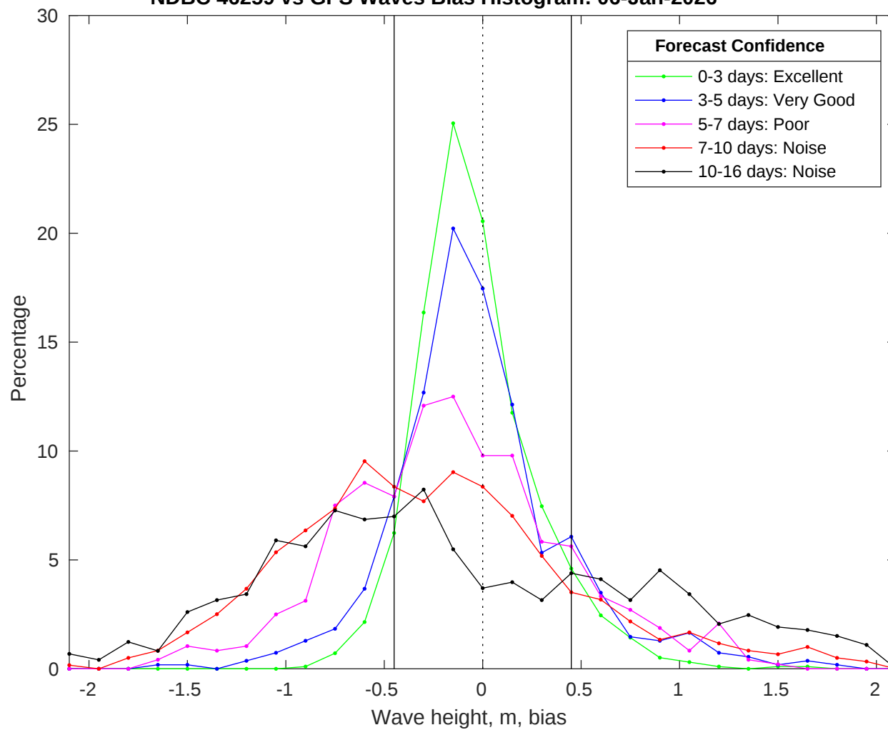
NDBC 46259 vs GFS Waves Bias Histogram: 06-Jan-2026
