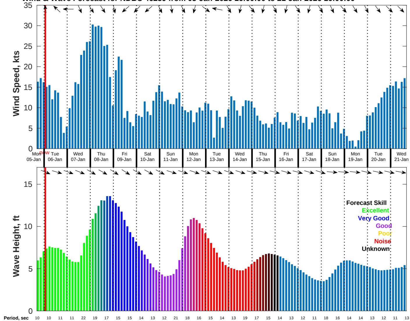
Wind & Wave Forecast for NDBC 46259 from 05-Jan-2026 16:00:00 to 21-Jan-2026 16:00:00
