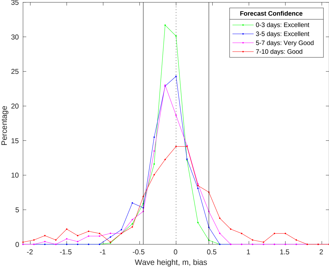
NDBC 51000 vs CMEMS Waves Bias Histogram: 06-Jan-2026
