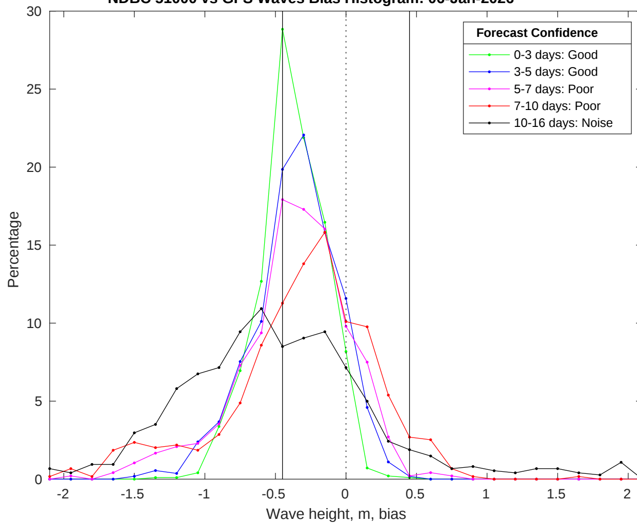
NDBC 51000 vs GFS Waves Bias Histogram: 06-Jan-2026
