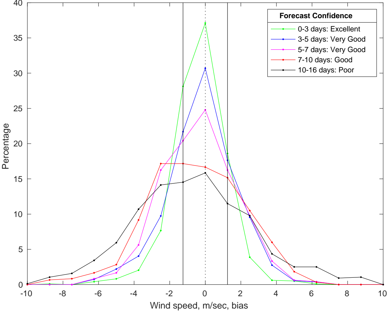
NDBC 51000 vs GFS Winds Bias Histogram: 06-Jan-2026
