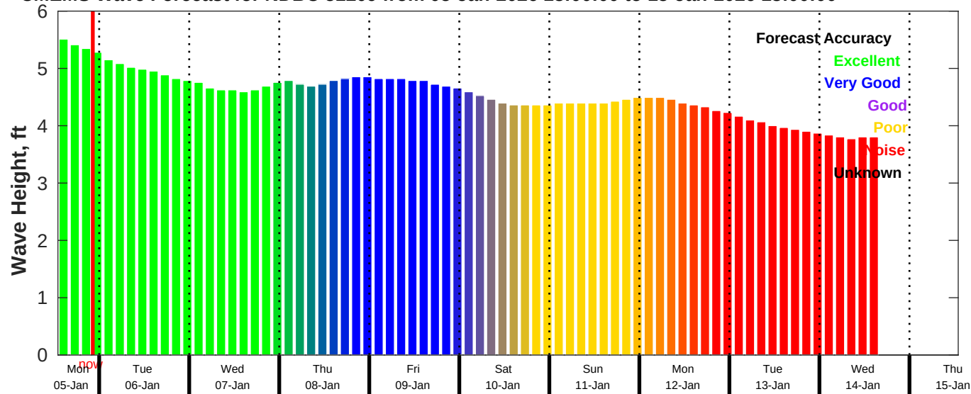
CMEMS Wave Forecast for NDBC 51209 from 05-Jan-2026 13:00:00 to 15-Jan-2026 13:00:00
