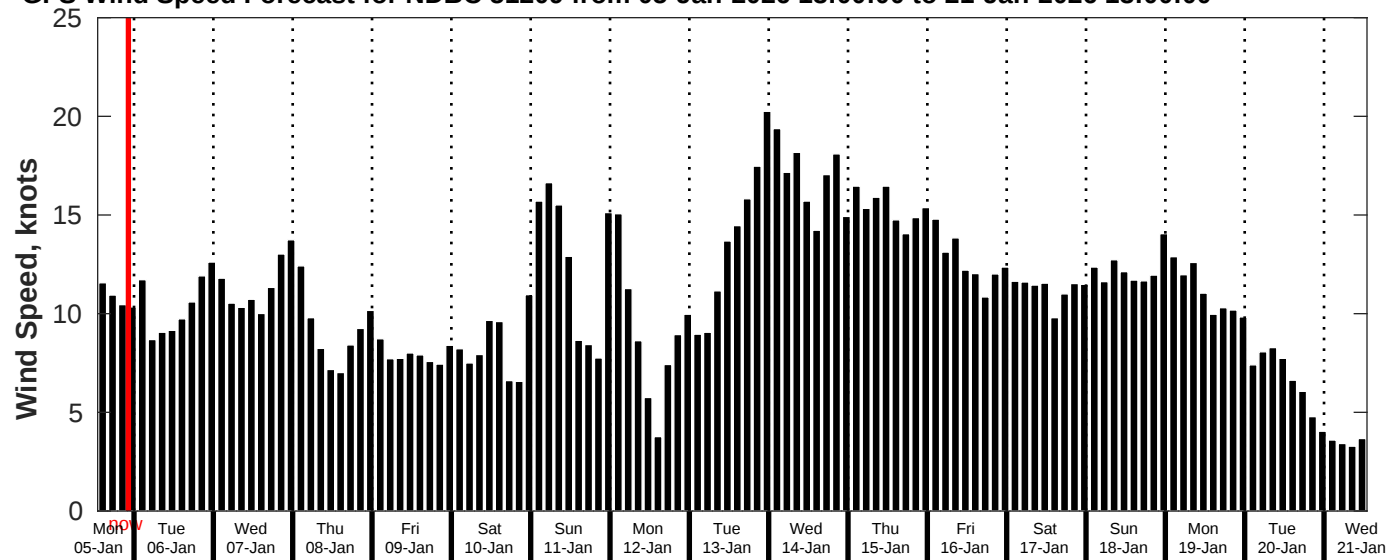
GFS Wind Speed Forecast for NDBC 51209 from 05-Jan-2026 13:00:00 to 21-Jan-2026 13:00:00
