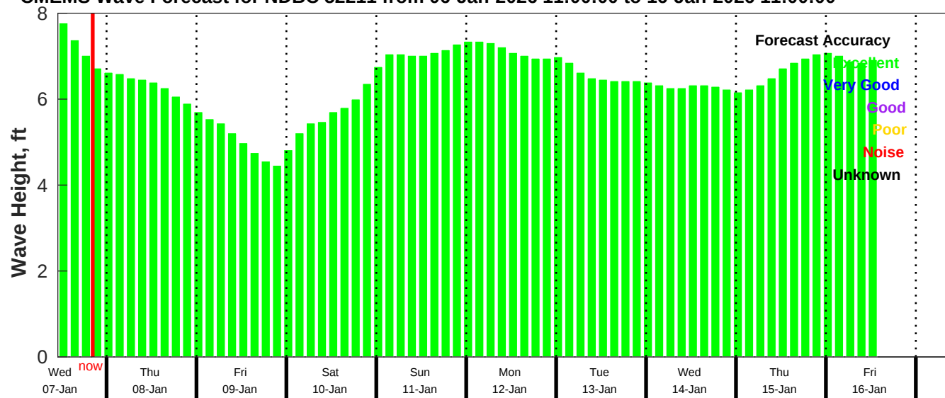
CMEMS Wave Forecast for NDBC 52211 from 06-Jan-2026 11:00:00 to 16-Jan-2026 11:00:00
