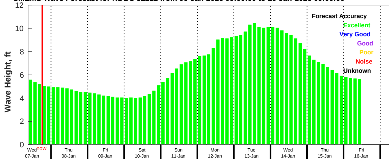
CMEMS Wave Forecast for NDBC 52212 from 06-Jan-2026 09:00:00 to 16-Jan-2026 09:00:00
