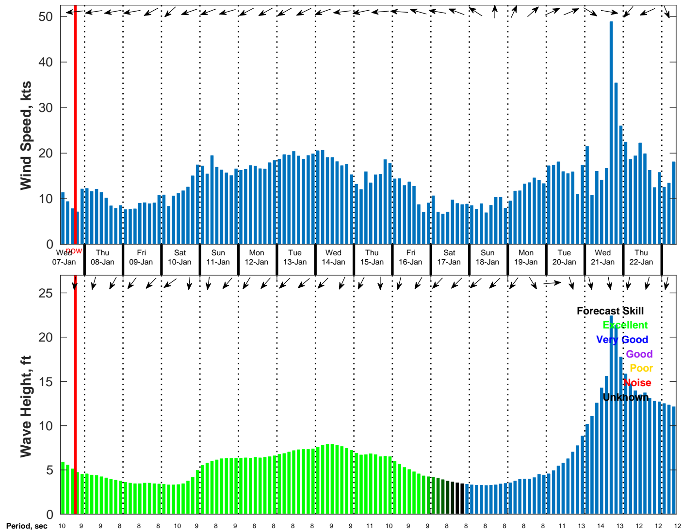
Wind & Wave Forecast for NDBC 52212 from 06-Jan-2026 09:00:00 to 22-Jan-2026 09:00:00
