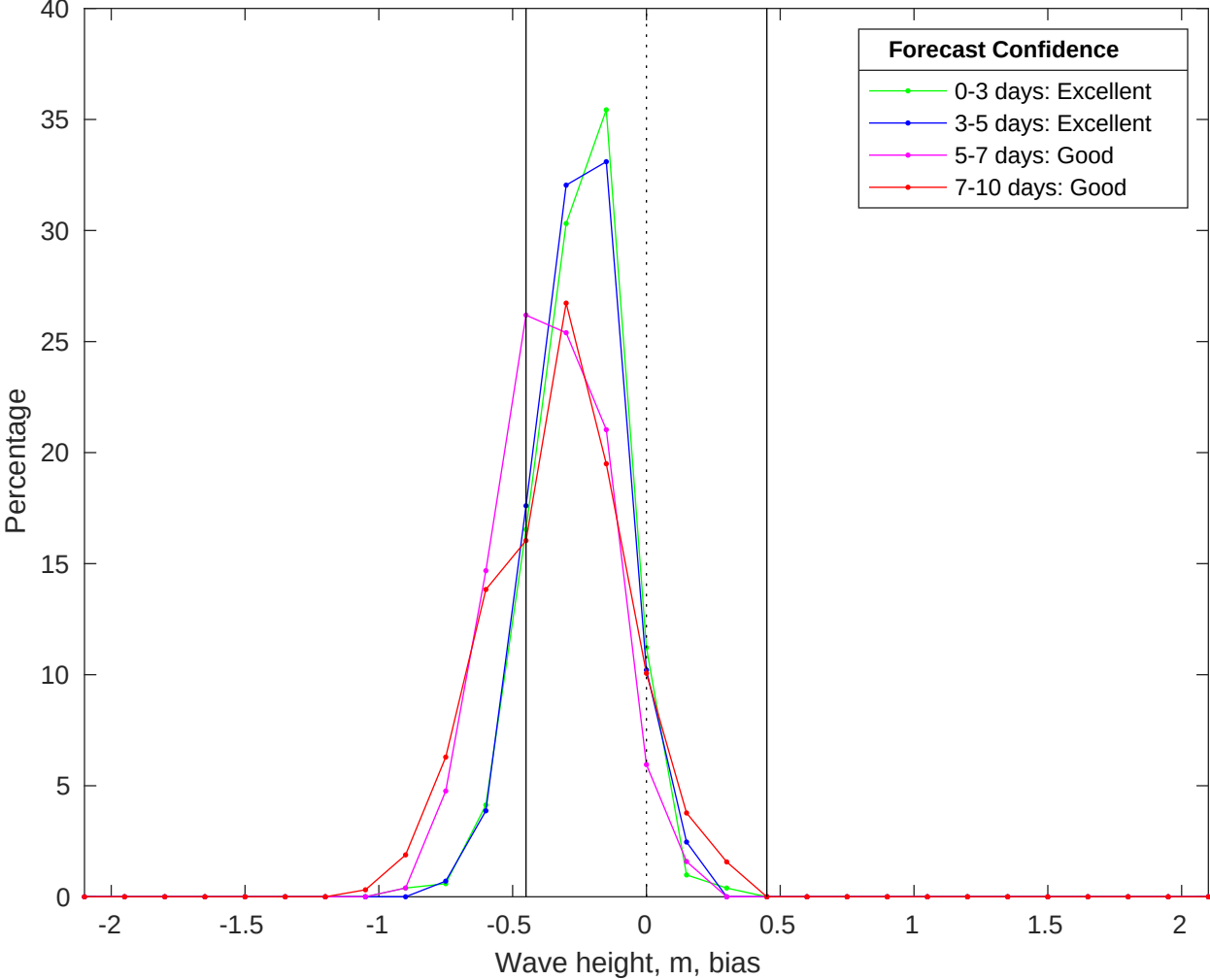
NDBC 52213 vs CMEMS Waves Bias Histogram: 06-Jan-2026
