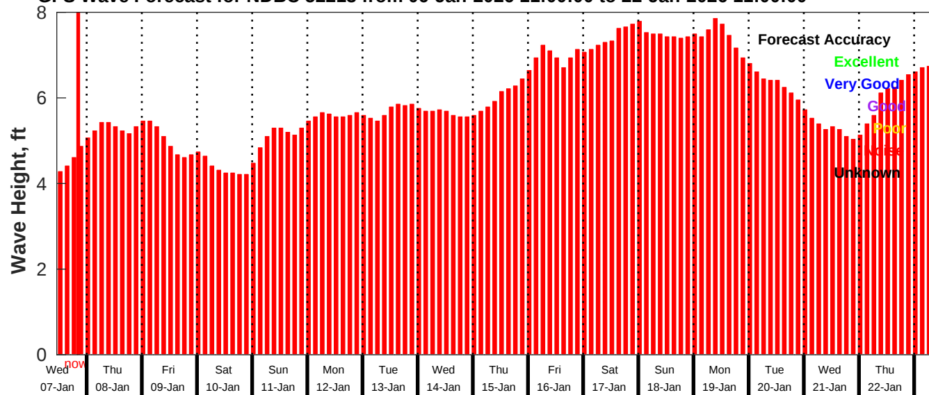
GFS Wave Forecast for NDBC 52213 from 06-Jan-2026 11:00:00 to 22-Jan-2026 11:00:00
