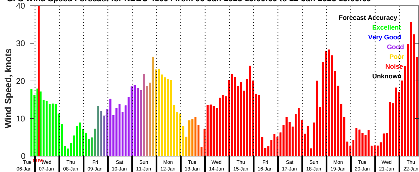
GFS Wind Speed Forecast for NDBC 41004 from 06-Jan-2026 19:00:00 to 22-Jan-2026 19:00:00
