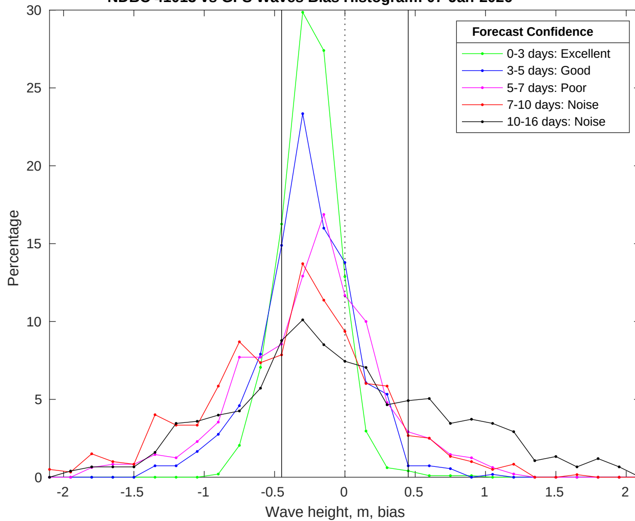
NDBC 41013 vs GFS Waves Bias Histogram: 07-Jan-2026
