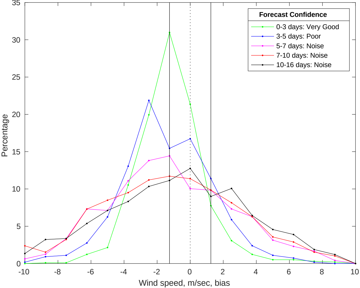
NDBC 41013 vs GFS Winds Bias Histogram: 07-Jan-2026
