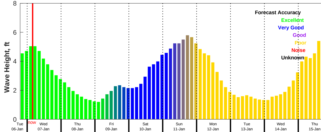
CMEMS Wave Forecast for NDBC 41013 from 06-Jan-2026 19:00:00 to 15-Jan-2026 19:00:00
