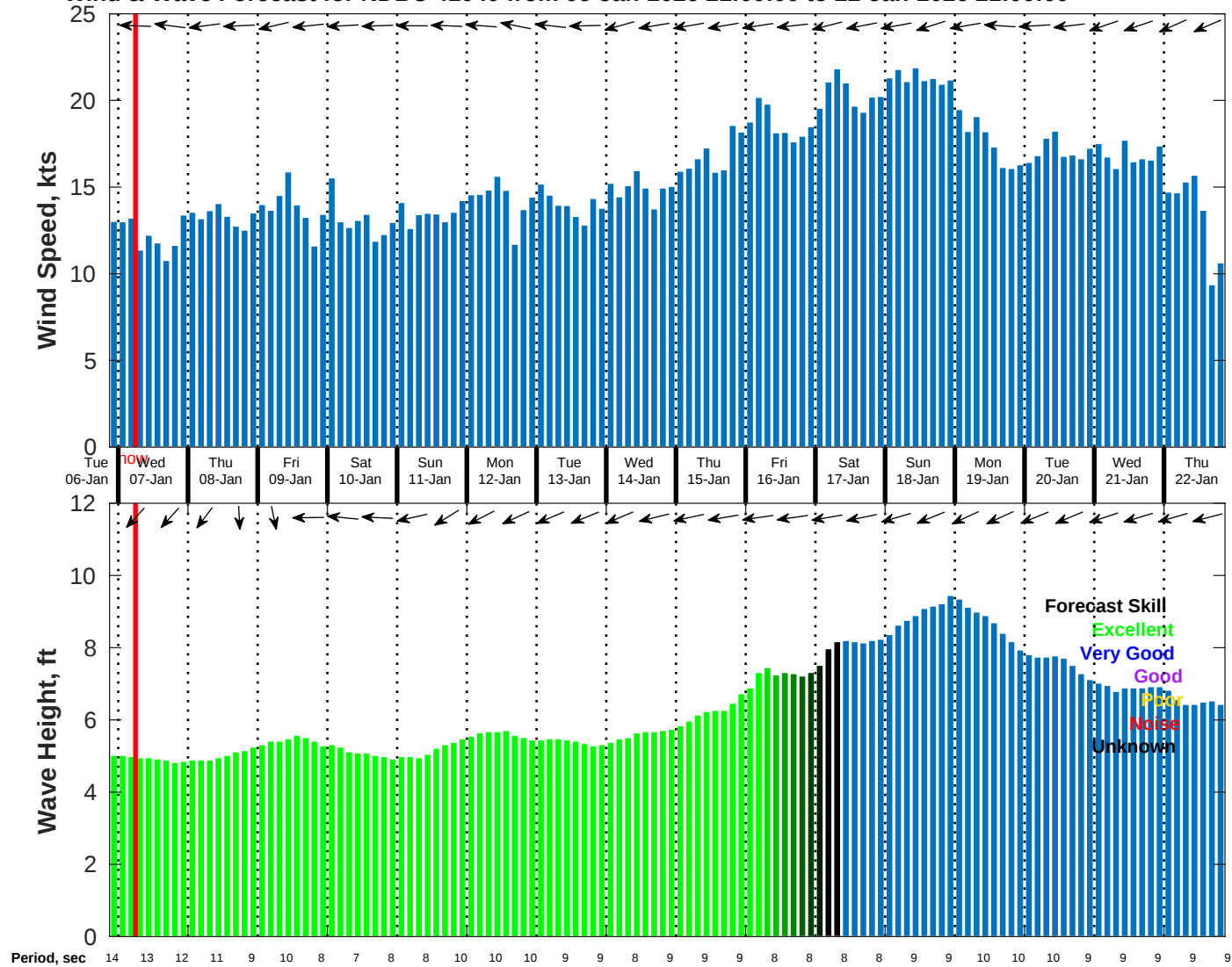
Wind & Wave Forecast for NDBC 41040 from 06-Jan-2026 21:00:00 to 22-Jan-2026 21:00:00
