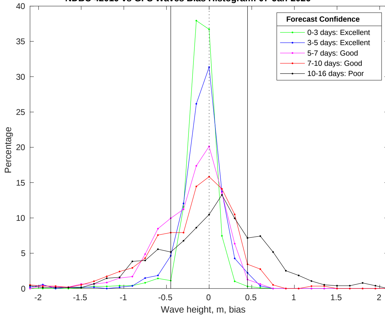
NDBC 42019 vs GFS Waves Bias Histogram: 07-Jan-2026
