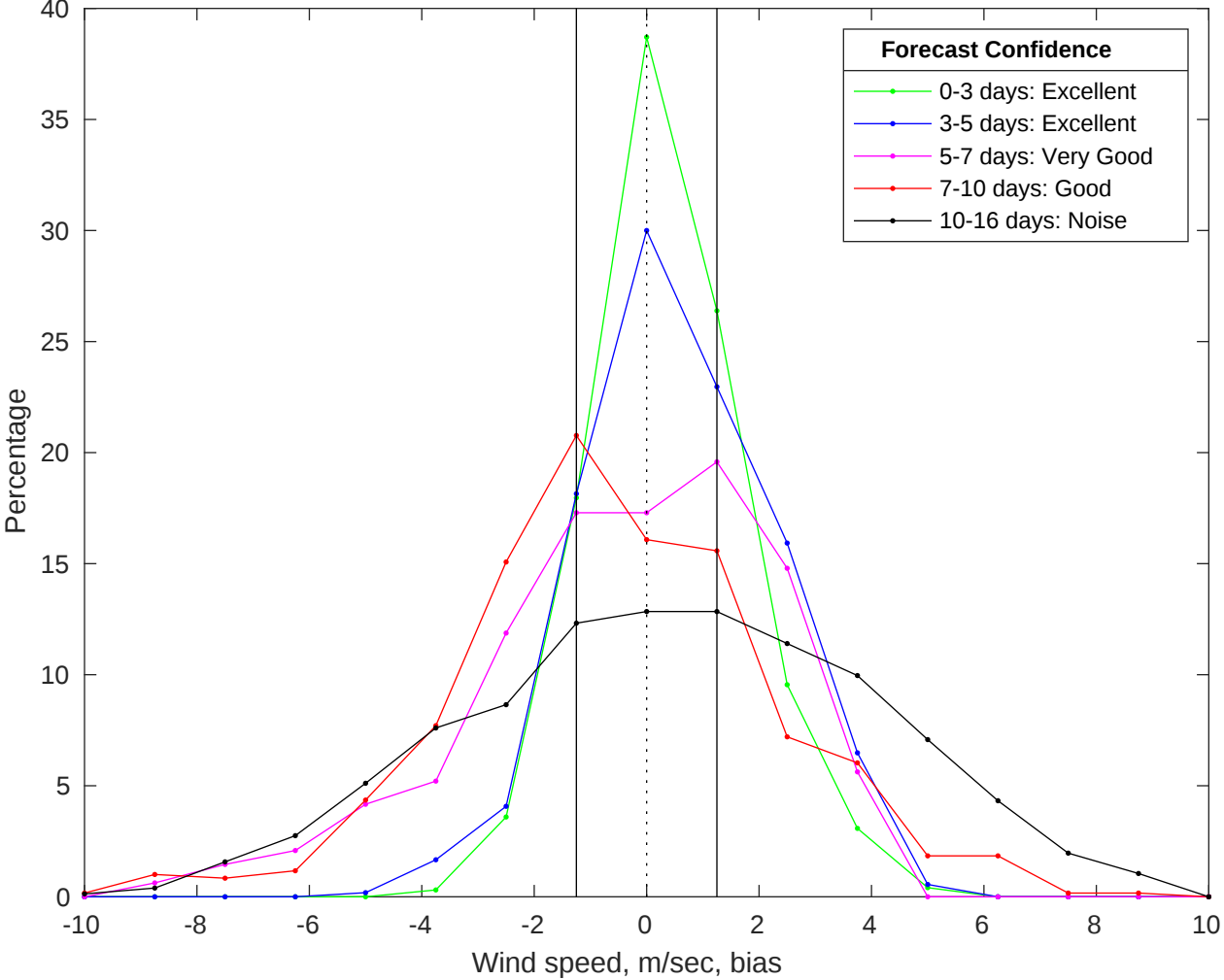
NDBC 42019 vs GFS Winds Bias Histogram: 07-Jan-2026
