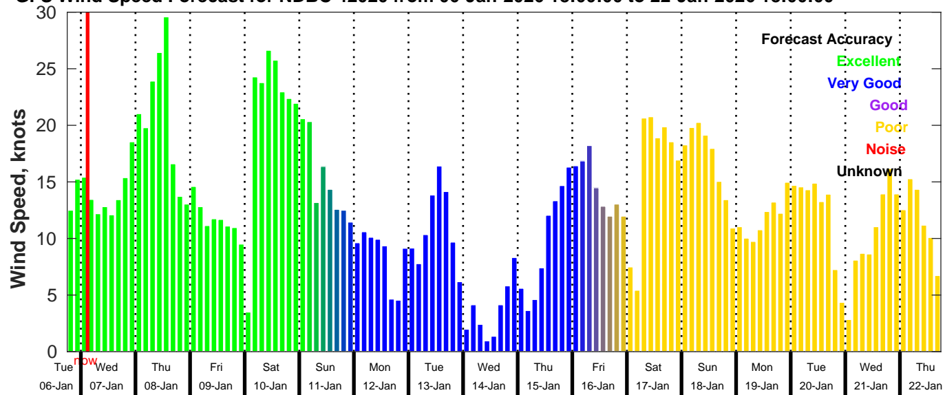
GFS Wind Speed Forecast for NDBC 42020 from 06-Jan-2026 18:00:00 to 22-Jan-2026 18:00:00
