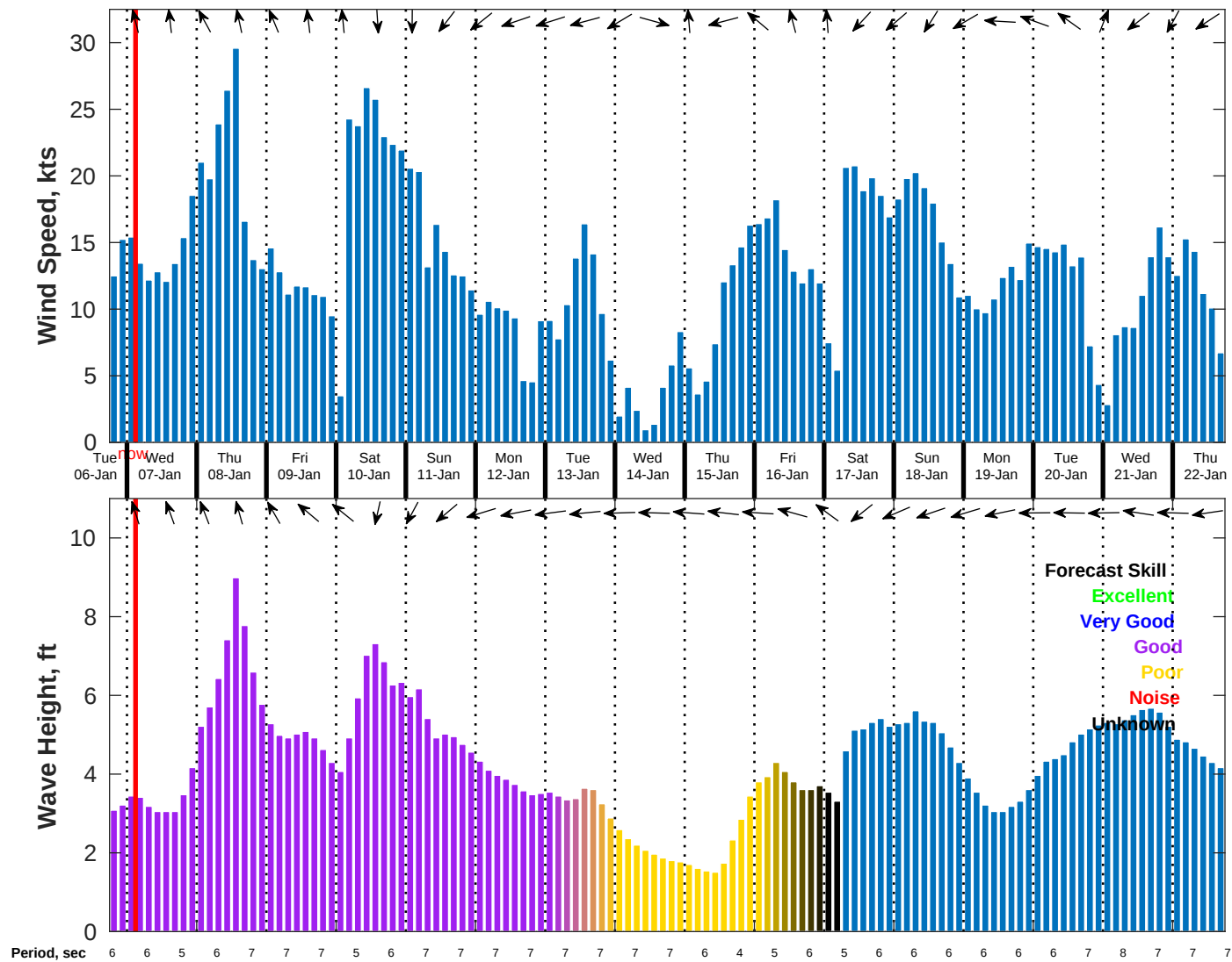
Wind & Wave Forecast for NDBC 42020 from 06-Jan-2026 18:00:00 to 22-Jan-2026 18:00:00
