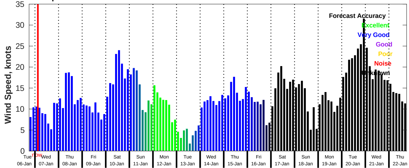
GFS Wind Speed Forecast for NDBC 42035 from 06-Jan-2026 18:00:00 to 22-Jan-2026 18:00:00
