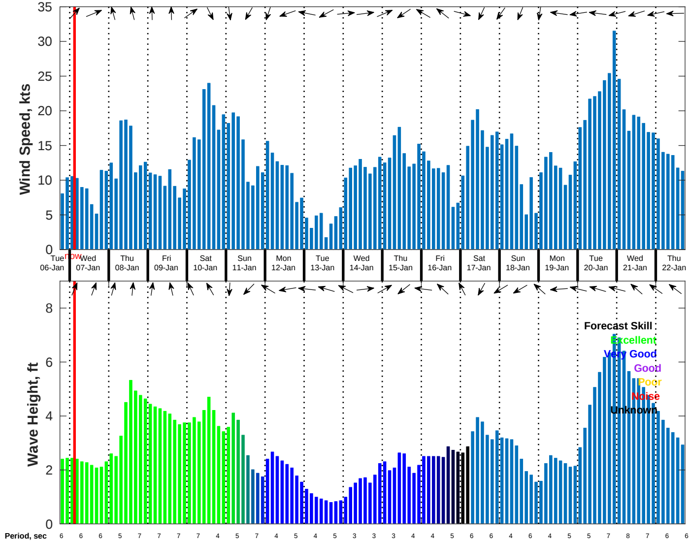
Wind & Wave Forecast for NDBC 42035 from 06-Jan-2026 18:00:00 to 22-Jan-2026 18:00:00
