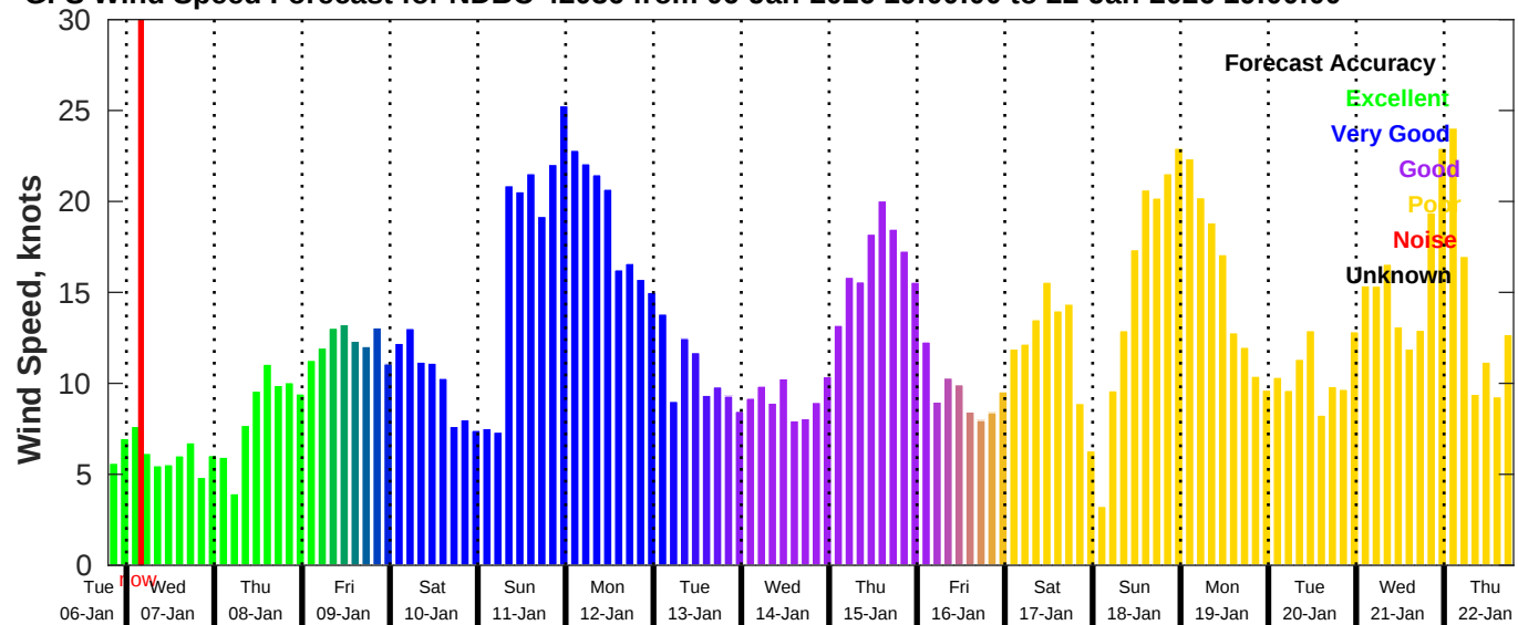
GFS Wind Speed Forecast for NDBC 42036 from 06-Jan-2026 19:00:00 to 22-Jan-2026 19:00:00
