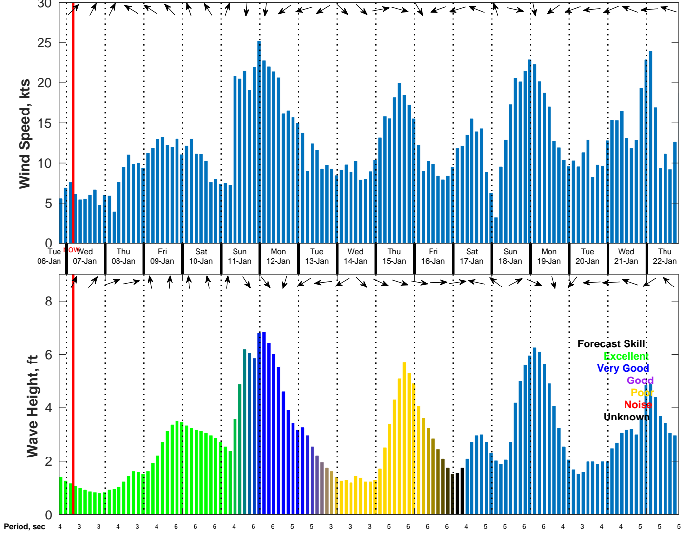
Wind & Wave Forecast for NDBC 42036 from 06-Jan-2026 19:00:00 to 22-Jan-2026 19:00:00
