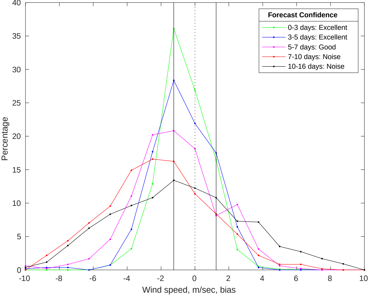
NDBC 42040 vs GFS Winds Bias Histogram: 07-Jan-2026
