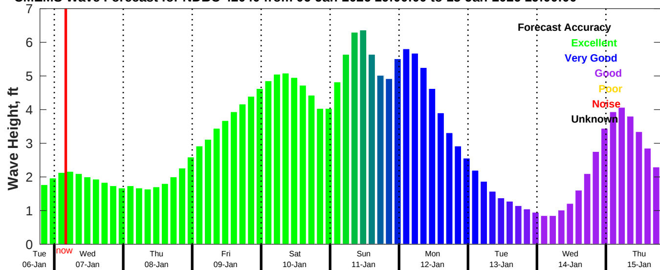
CMEMS Wave Forecast for NDBC 42040 from 06-Jan-2026 19:00:00 to 15-Jan-2026 19:00:00
