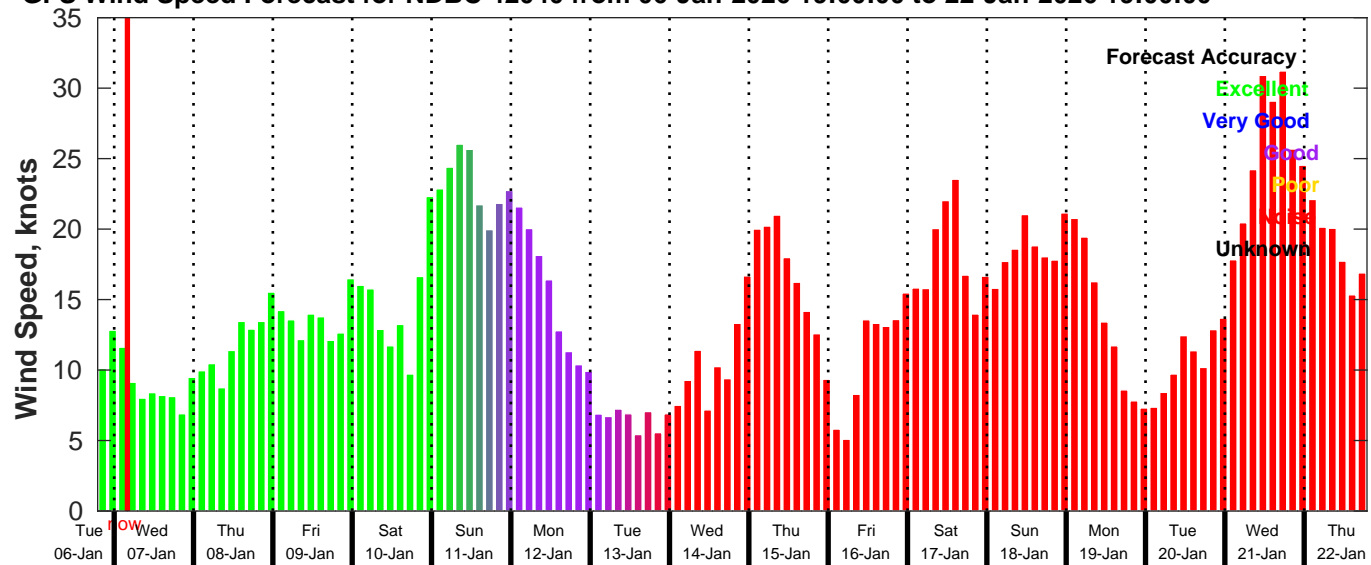
GFS Wind Speed Forecast for NDBC 42040 from 06-Jan-2026 19:00:00 to 22-Jan-2026 19:00:00
