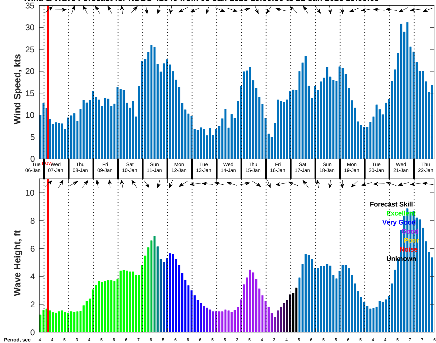
Wind & Wave Forecast for NDBC 42040 from 06-Jan-2026 19:00:00 to 22-Jan-2026 19:00:00
