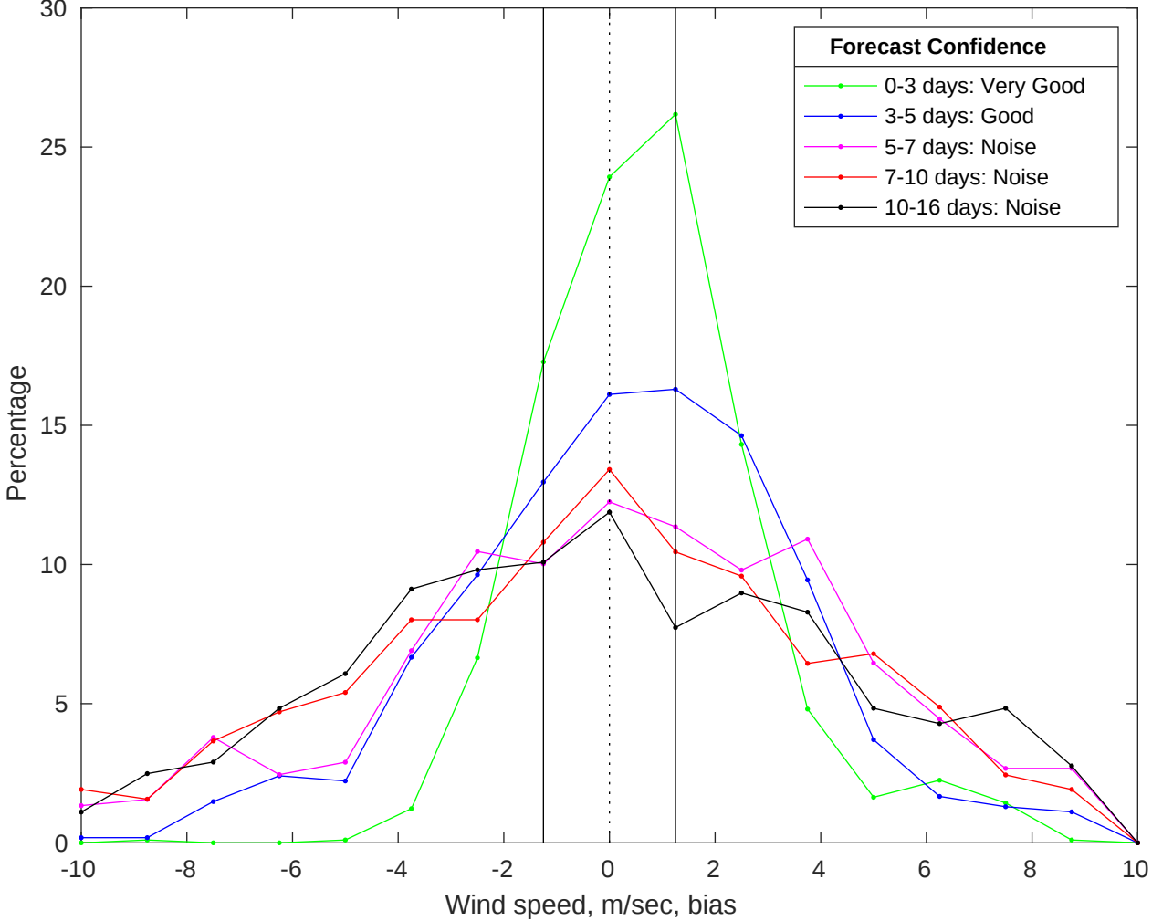
NDBC 44008 vs GFS Winds Bias Histogram: 07-Jan-2026
