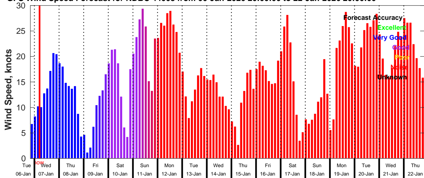
GFS Wind Speed Forecast for NDBC 44008 from 06-Jan-2026 20:00:00 to 22-Jan-2026 20:00:00
