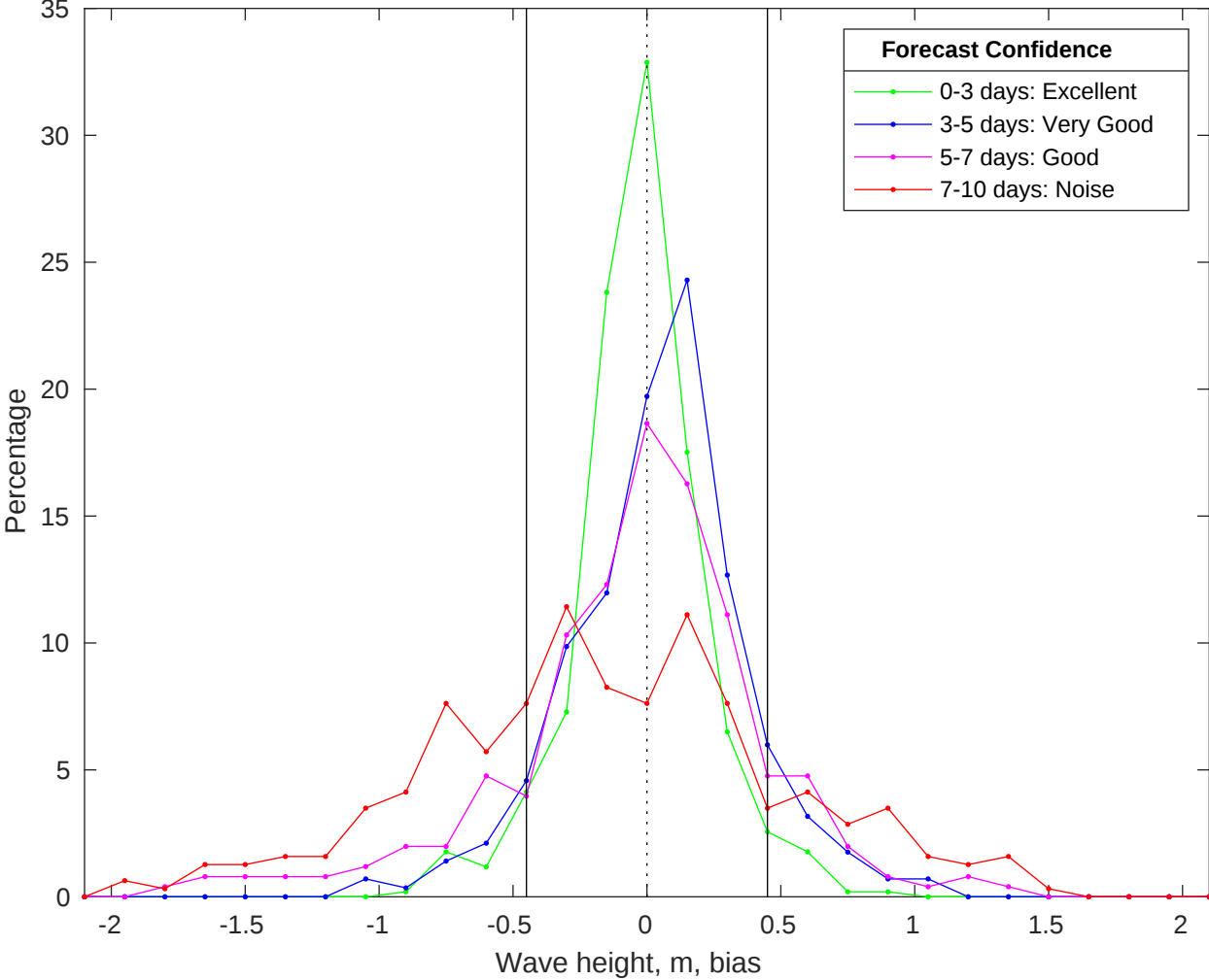
NDBC 46011 vs CMEMS Waves Bias Histogram: 07-Jan-2026
