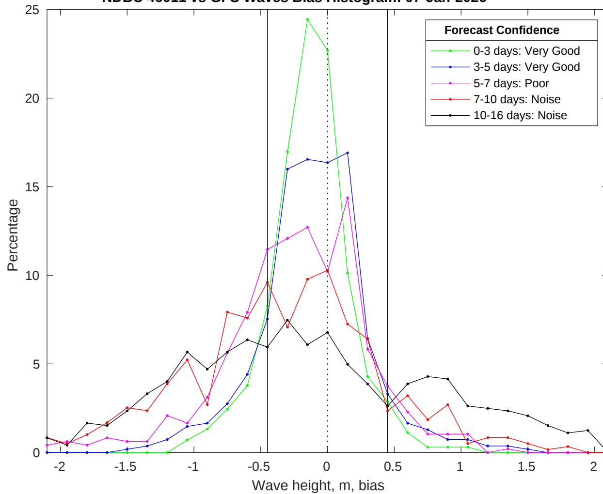
NDBC 46011 vs GFS Waves Bias Histogram: 07-Jan-2026
