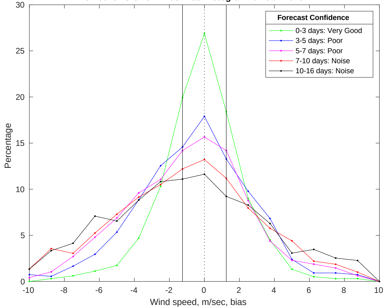
NDBC 46028 vs GFS Winds Bias Histogram: 07-Jan-2026
