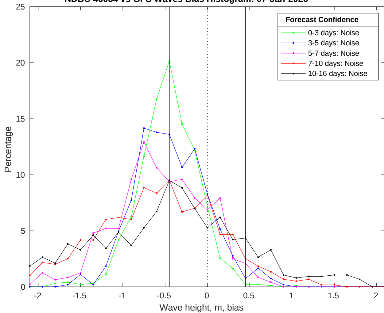
NDBC 46054 vs GFS Waves Bias Histogram: 07-Jan-2026
