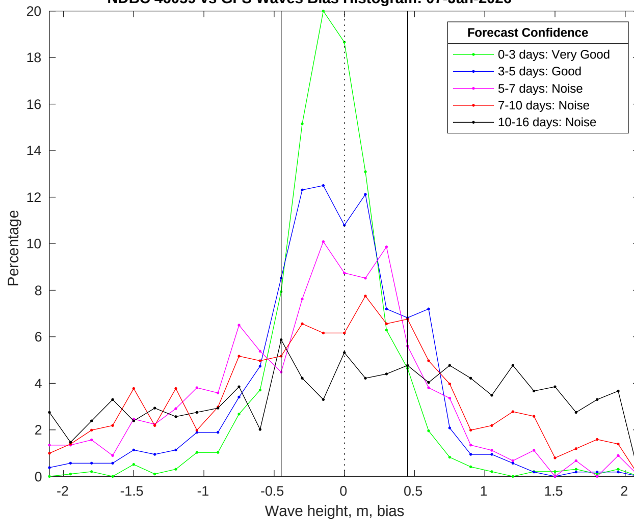
NDBC 46059 vs GFS Waves Bias Histogram: 07-Jan-2026
