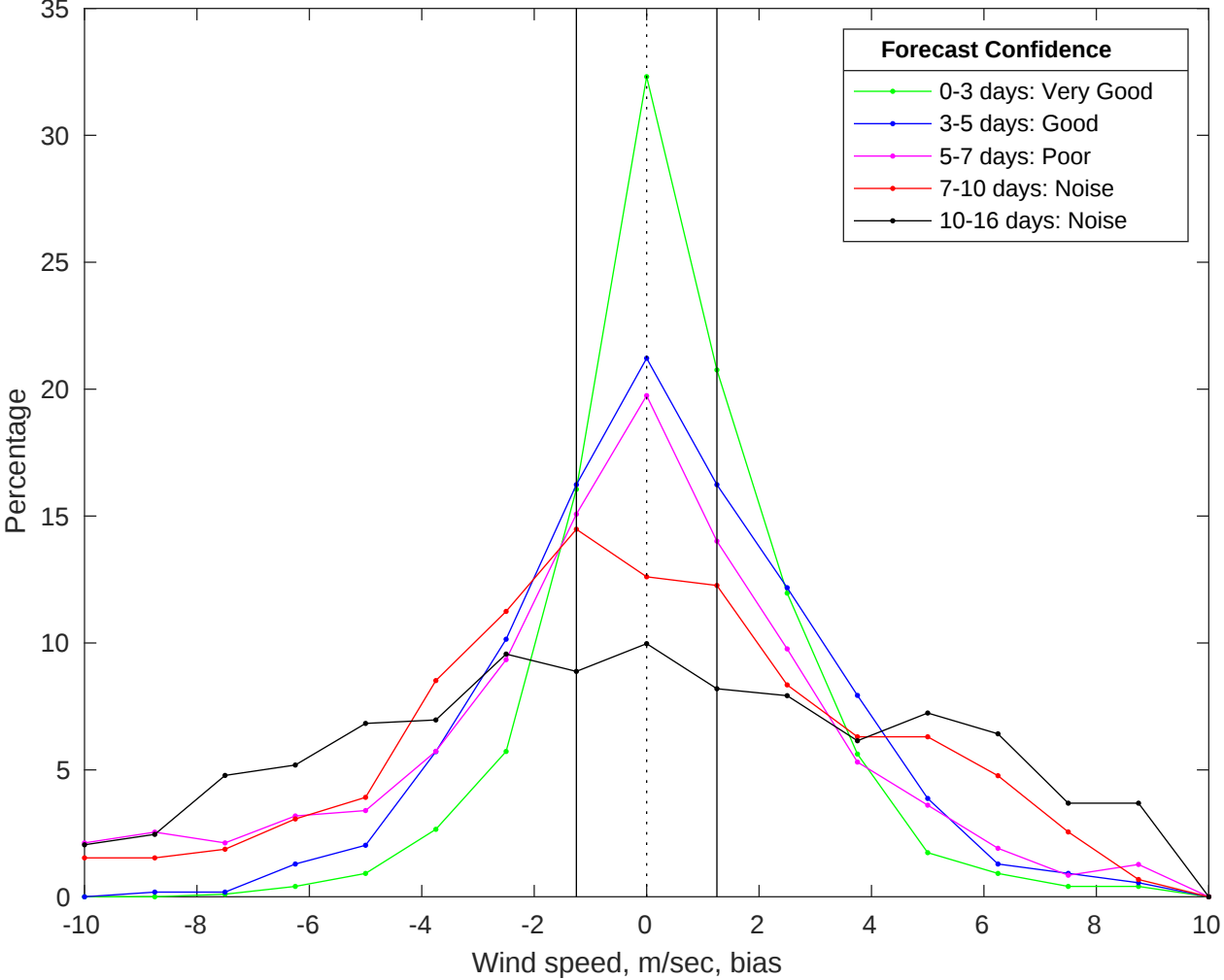
NDBC 46059 vs GFS Winds Bias Histogram: 07-Jan-2026
