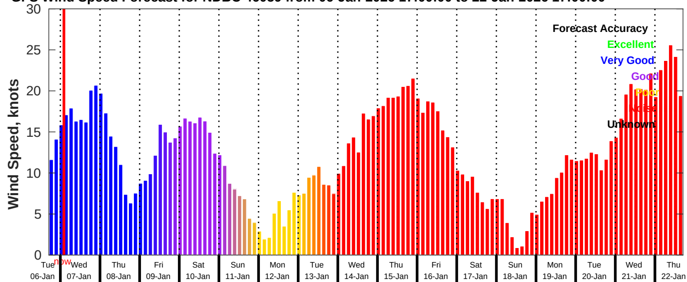
GFS Wind Speed Forecast for NDBC 46059 from 06-Jan-2026 17:00:00 to 22-Jan-2026 17:00:00
