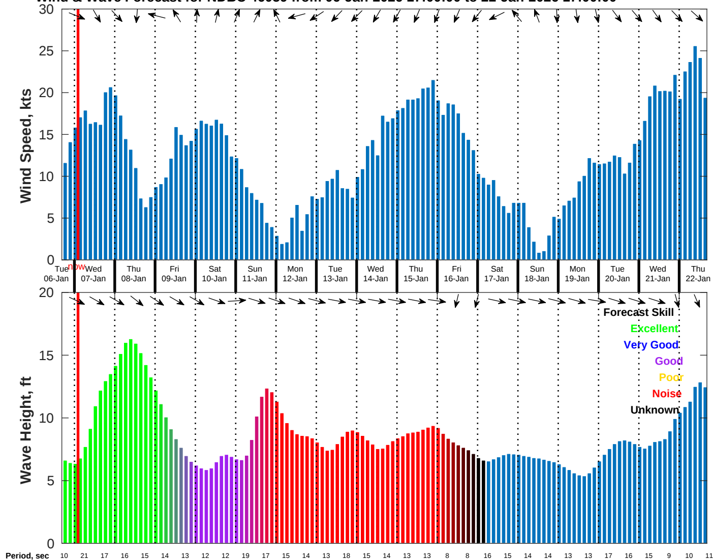
Wind & Wave Forecast for NDBC 46059 from 06-Jan-2026 17:00:00 to 22-Jan-2026 17:00:00
