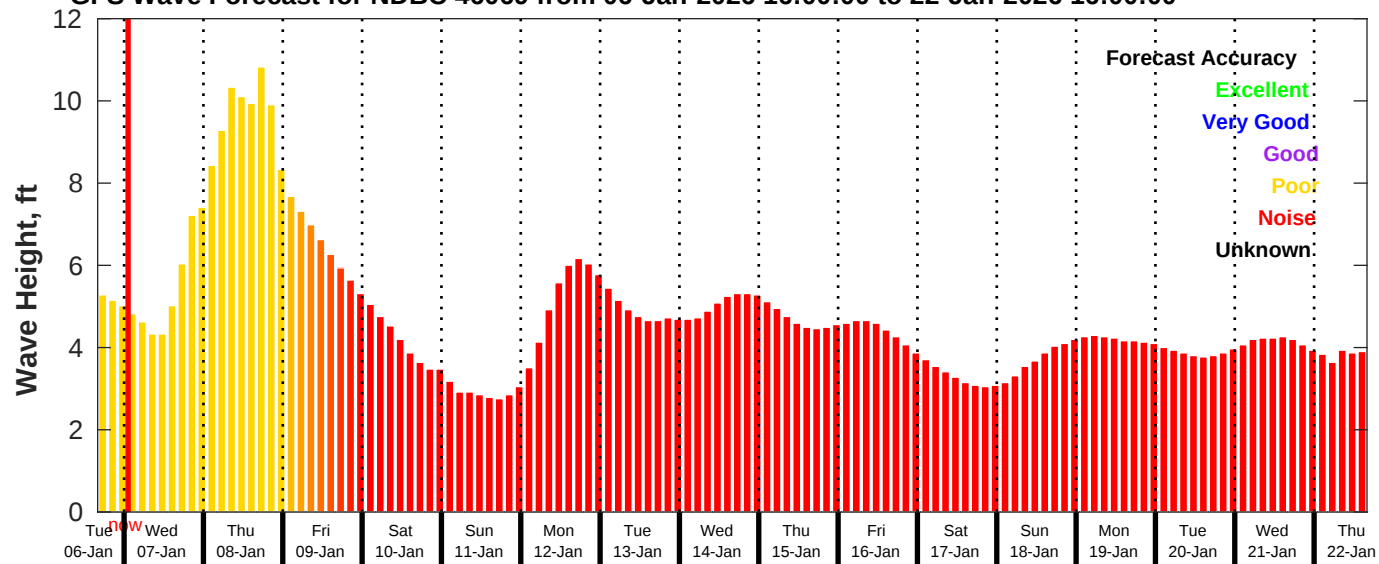
GFS Wave Forecast for NDBC 46069 from 06-Jan-2026 16:00:00 to 22-Jan-2026 16:00:00
