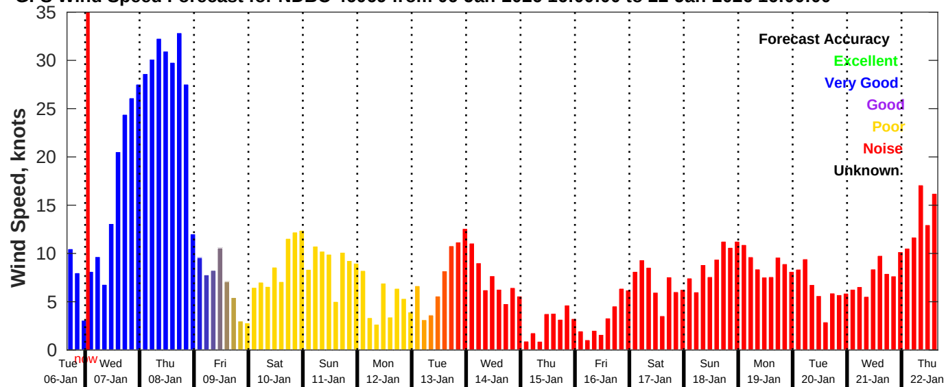
GFS Wind Speed Forecast for NDBC 46069 from 06-Jan-2026 16:00:00 to 22-Jan-2026 16:00:00
