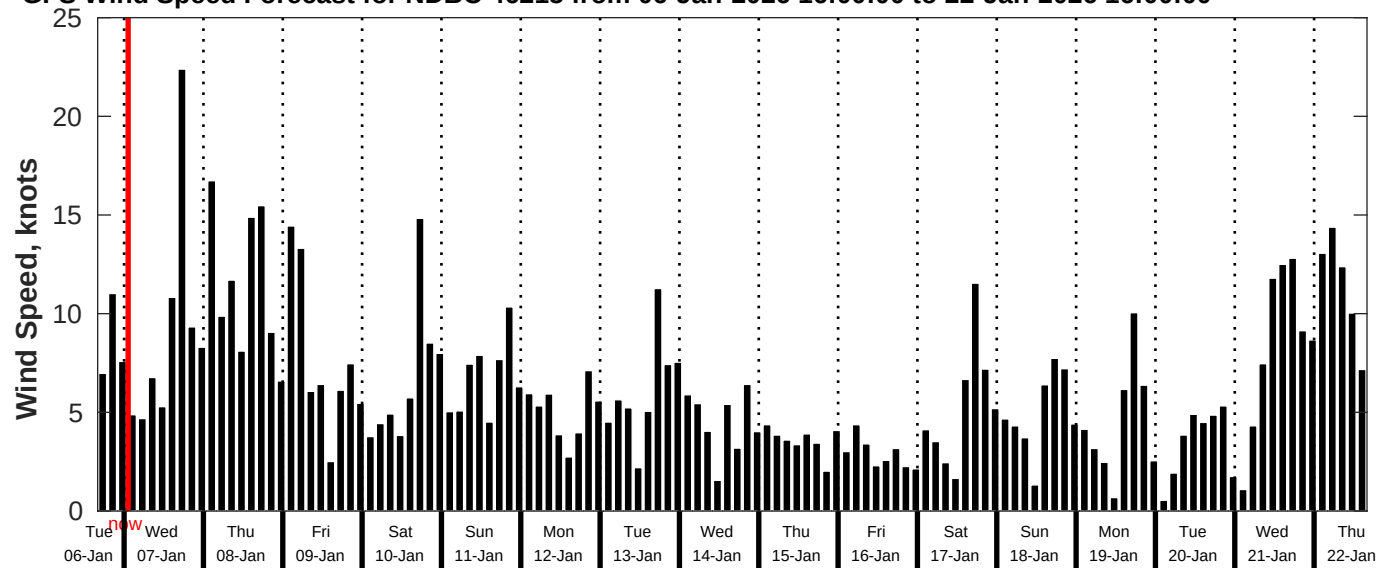
GFS Wind Speed Forecast for NDBC 46215 from 06-Jan-2026 16:00:00 to 22-Jan-2026 16:00:00
