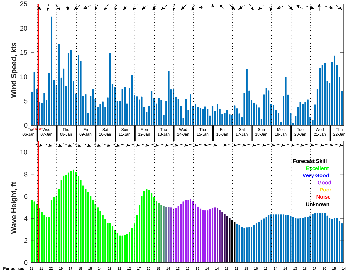
Wind & Wave Forecast for NDBC 46215 from 06-Jan-2026 16:00:00 to 22-Jan-2026 16:00:00
